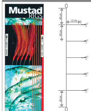
RED/YELLOW POLLACK AND MACKEREL TRACES T57 SIZE 1/0, 3/0
