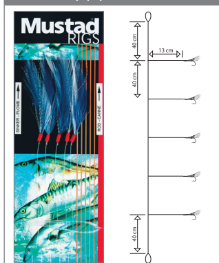
BLUE/WHITE POLLACK AND MACKEREL TRACES T58 SIZE 1/0, 3/0
