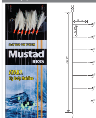
FEATHER RIG T82 SIZE 2, 4, 6
