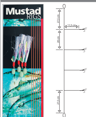
SILVER FLASHER T53 SIZE 3/0
