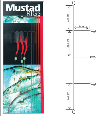
HOKKAI TEMPTER RIG, RED T17C SIZE 6/0
