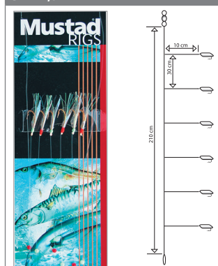
FISHSKIN BI-COLOR T81 SIZE 4, 6
