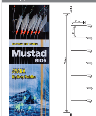
PISCATOR RIG T80 SIZE 2, 4, 6
